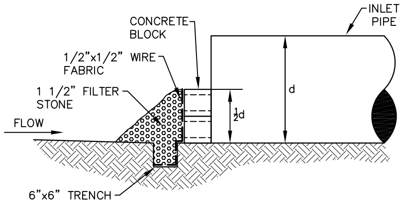
SECTION VIEW
